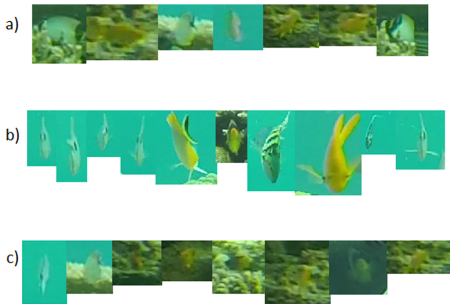
Fig. 2. Samples of thumbnails recognized by the CNN model and not recognized by humans (a), samples of thumbnails recognized by humans and not recognized by the CNN model (b) and sample of thumbnails misidentified by both humans and the CNN model (c).
